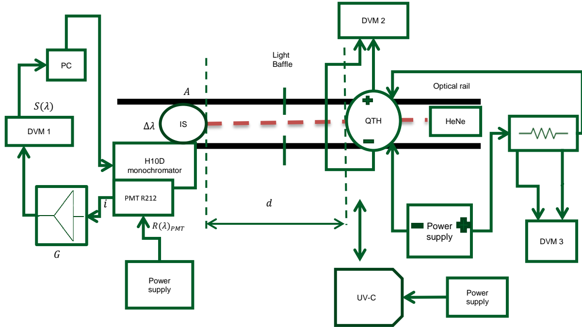
Figure 1: The measurement setup of the spectral irradiance lamp calibrations at NMISA. The setup makes use of a substitution method where one lamp is measured at a time.
