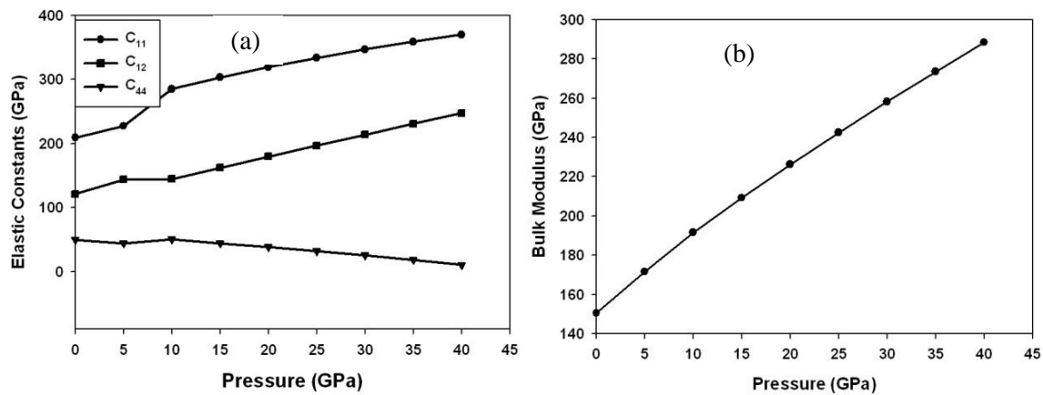
Figure 3: The variation of the (a) elastic constants and (b) Bulk modulus as a function of increasing pressure.
