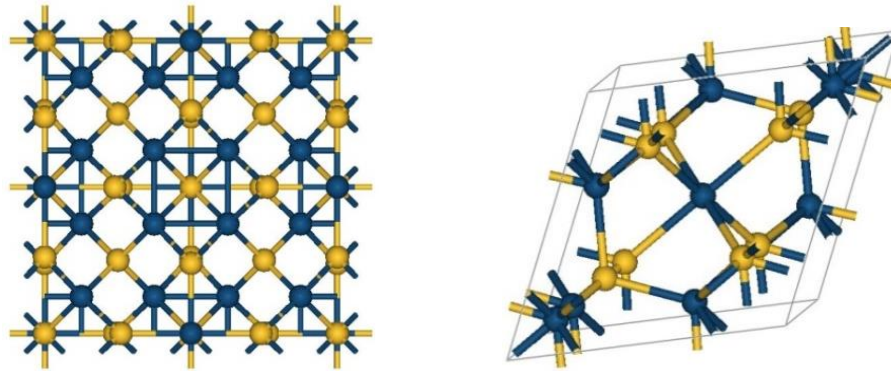
Figure 1: Conventional ( \text{Ir}_{36}\text{S}_{32} ) and primitive ( \text{Ir}_9\text{S}_8 ) unit cell of pentlandite structure. Blue and yellow spheres represent metal (Ir) and sulphur (S) atoms respectively.
