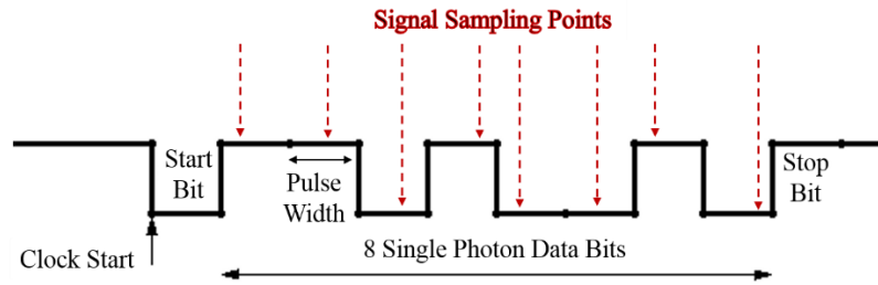
Figure 2. Asynchronous transmission begins with a Start bit which serves as the synchronisation indicator. The pulse width of each bit is agreed upon before the transmission begins and the receiver is able to measure the 8 data bits following the Start bit. The Stop bit indicates that the data has stopped, pending the transmission of another Start bit.
