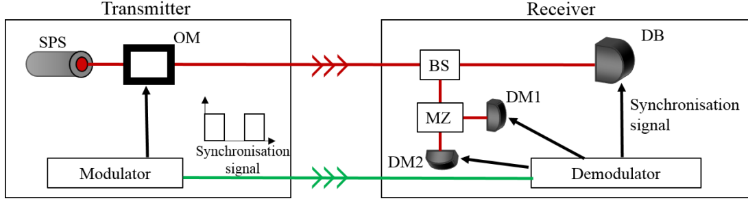
Figure 1. A schematic of the COW protocol detailing the transmitter and receiver modules. The transmitter includes a faint, coherent laser source, SPS, coupled with an external optical modulator, OM, used to create the bit encoding. The transmitter also includes a synchronisation modulator and additional electronics and on-board memory required for post-processing. The receiver module requires a beam splitter, BS, to create two separate optical paths from the incoming bit stream. The first path serves as the detection line and requires a single photon detector, DB, which measures incoming photons to create the raw key. The second path of the beam splitter serves as the monitoring line. This path consists of a Mach-Zehnder interferometer, MZ, and single photon detectors at each output of the interferometer, DM1 and DM2. The purpose of the interferometer is to confirm the coherence between two consecutive decoy pulses. A break in coherence infers the presence of an eavesdropper. The demodulator receives the synchronisation signal and commands the gates of the single photon detectors DB, DM1 and DM2.
