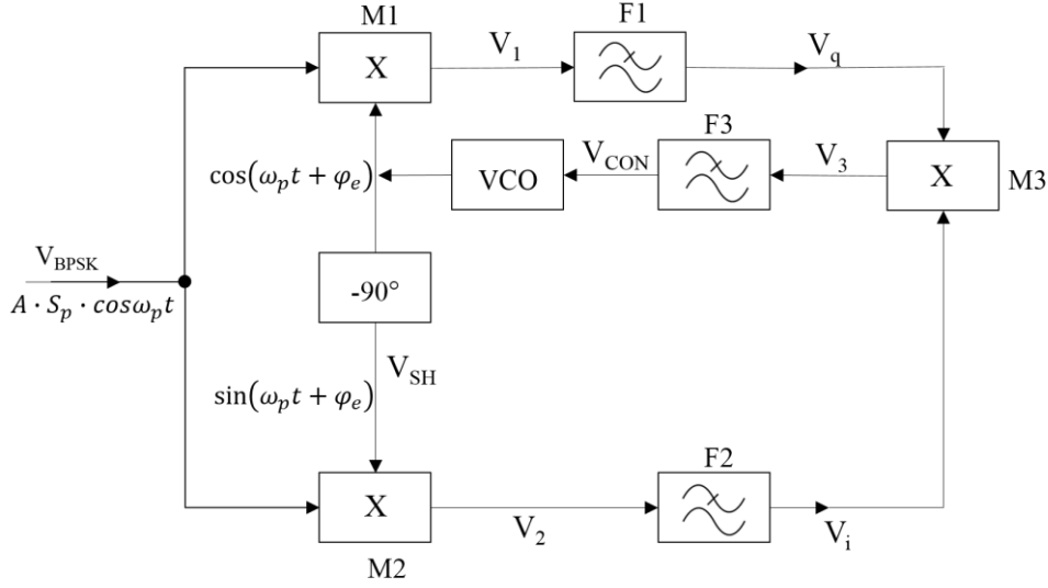
Figure 4. A diagram of the Costas loop, used to demodulate the BPSK signal. VCO is a voltage controlled oscillator which oscillates with the same frequency as the received V_{\text{BPSK}} signal. Any phase difference between the signals must be resolved. V_{\text{BPSK}} is multiplied by VCO at multiplier M1. VCO undergoes a -90^\circ phase shift and is multiplied to V_{\text{BPSK}} at M2. Both signals are passed through respective low pass filters F1 and F2 and are multiplied at M3. The resultant signal is passed through low pass filter F3 in order to remove any noise and is then applied to VCO to correct the phase difference. The signal from VCO can then be used to synchronise the receiver module.
