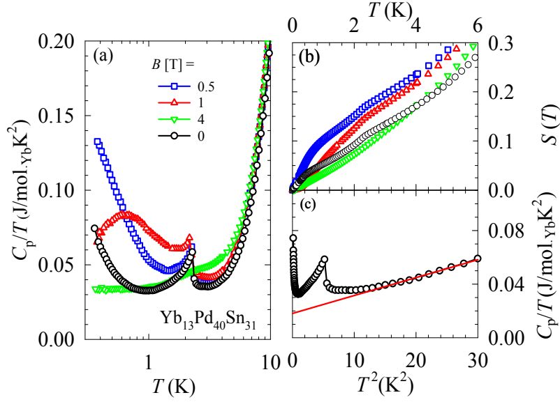
Figure 4. (a): Temperature dependence of the heat capacity for different applied magnetic fields. (b): Calculated entropy in different applied fields. (c): Low temperature region of the C_p/T vs T^2 dependence in zero field with a fit of the most linear region as discussed in the text.
