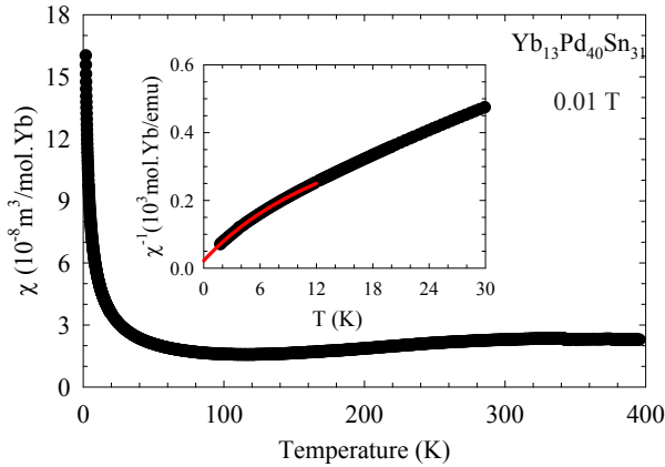
Figure 1. Temperature dependence of the magnetic susceptibility \chi(T) measured up to 400 K. The inset represents the least-squares fit of equation 1 to the low-region of \chi(T) with parameters as discussed in the text.
