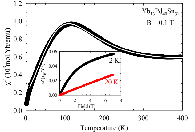
Figure 2. Temperature dependence of the inverse magnetic susceptibility \chi^{-1}(T) . The solid line represents the ICF fit of equation 3 as discussed in the text. Inset: magnetization isotherms in fields up to 7 T.
