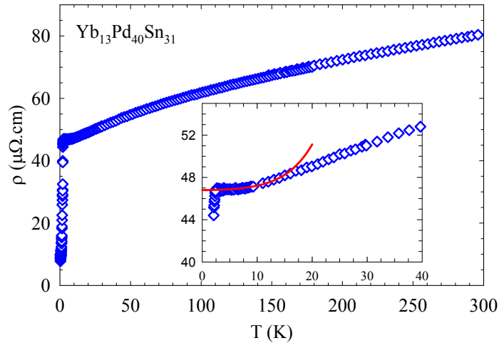
Figure 3. Temperature dependence of electrical resistivity. Inset: Low temperature region with a least-squares fit of the Fermi-liquid relation.
