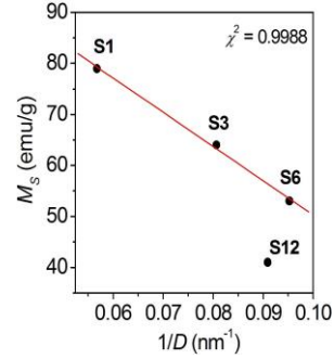
Figure 9. A fit to estimate M_s (bulk) and the thickness dead layer d .
