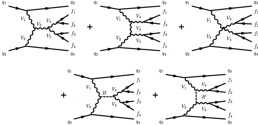
Figure 1. Representative Feynman diagrams of VVjj -EW production. The VBS scattering topology includes either a triple gauge coupling vertex, the t-channel exchange, a quartic boson coupling vertex or a Higgs boson exchange in the s- or t-channels. The lines are labelled by quarks (q), vector bosons (V) and fermions (f).
