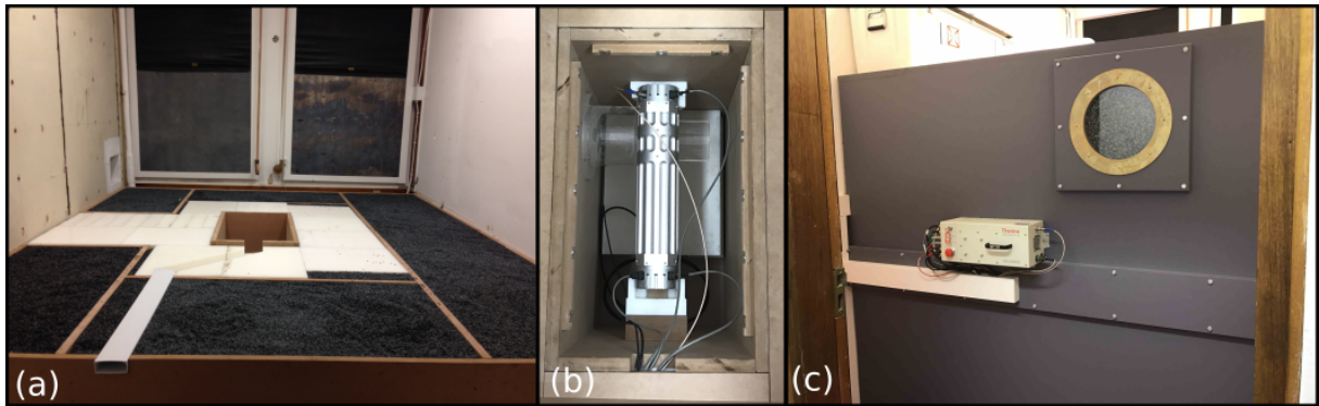
Figure 4. Photos of the neutron shielding (a) during and (c) after construction. The core component of the shielding are white blocks of HDPE, surrounded by the black HDPE beads. The neutron generator is situated in the central void as shown in photo (b). A neutron and gamma-ray sensitive monitor detector is installed underneath the STNG. The electronics have been separated from the generator and are installed outside the shielding as shown in photo (c). All generator and detector cables are routed into the control area. Note that the porthole visible in photo (c) serves no scientific function.
