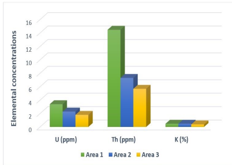
Figure 3. Mean values of ^{238}\text{U} , ^{232}\text{Th} , ^{40}\text{K}
