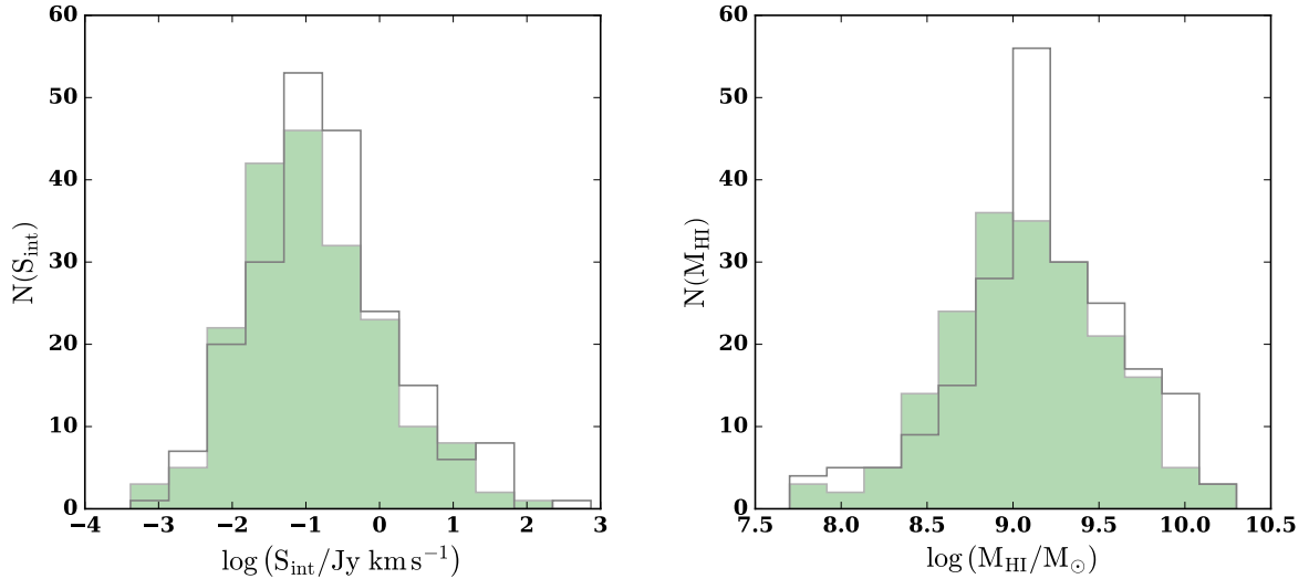
Figure 2. HI parameter comparison between visual and semi-automated galaxy detection in the WSRT PP HI data cube. Green indicates the HI distribution based on visual catalogue, whereas the open grey histogram is based on semi-automated results. Left panel: logarithm distribution of integrated flux \log(S_{\text{int}}/\text{Jy km s}^{-1}) , right panel: the logarithmic distribution of HI mass \log(M_{\text{HI}}/M_{\odot}) .
