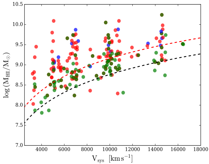
Figure 1. The logarithm of total HI mass of all detected galaxies (through visual inspection) as a function of radial velocity. The red and the black dashed lines, show the HI mass limit of the WSRT dataset assuming a 3\sigma detection with 100 and 250 \text{km s}^{-1} linewidths, respectively. The green dots indicate detected galaxies with measured linewidths less than 100 \text{km s}^{-1} . The red dots indicate galaxies of linewidths between 100 & 250 \text{km s}^{-1} . Whereas the blue dots show galaxies with linewidths greater than 250 \text{km s}^{-1} .
