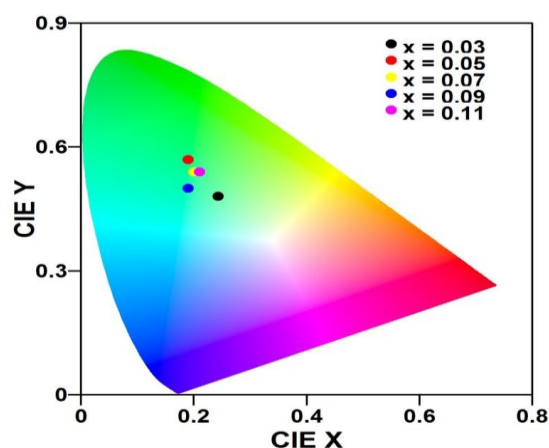
Figure 5: CIE chromaticity diagram of \text{BaB}_8\text{O}_{13} doped different concentrations of \text{Ce}^{3+} .
