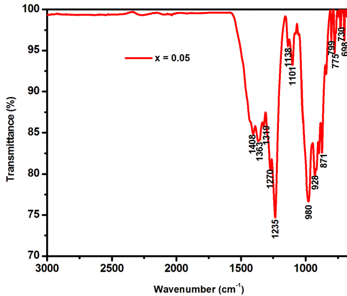
Figure 2. Room temperature FTIR spectrum of BaB 8 O 13 :0.05Ce 3+ phosphor.
