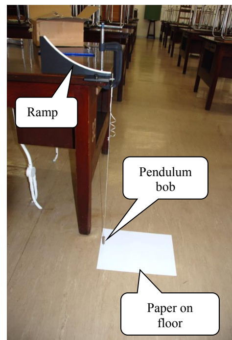
Figure 3. Collision experiment apparatus.
