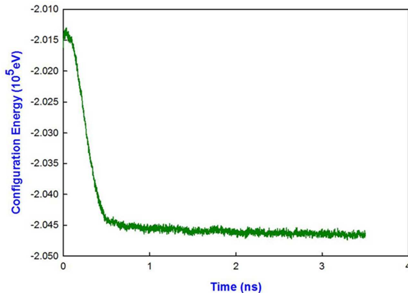
Figure 2. Calculated configuration energy as a function of time for the lithiated nanostructure of \text{TiO}_2 .
