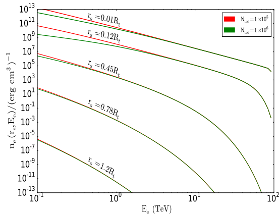
Figure 2: The steady-state particle spectrum as a function of particle energies E_e for different radii r_s .
