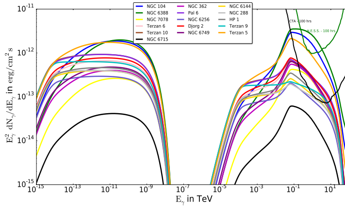
Figure 4: Predicted SED E_\gamma^2 dN_\gamma/dE_\gamma in \text{erg cm}^{-2}\text{s}^{-1} for 15 non-detected GCs and for Terzan 5. The two components represent the SR and IC spectra. The H.E.S.S. and CTA sensitivities (for 100 hours) are also shown.
