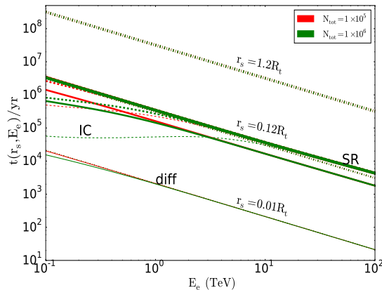
Figure 1: Timescales as a function of energy for diffusion (dotted lines), radiation losses (dashed lines), and the effective scale (solid lines). Thicker lines represent larger radii. The colours represent different values of N_{\text{tot}} as noted in the legend.
