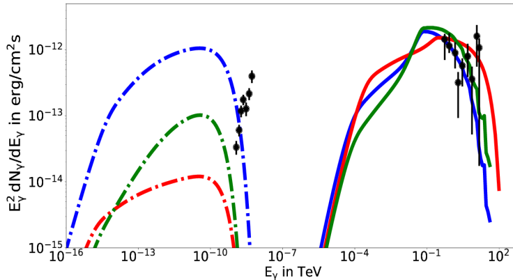
Figure 3: The SED for Terzan 5 indicating the predicted SR (integrated between 55' < r_s < 174' to match Chandra FOV, the dash-dotted lines) for the inner part of the source and IC (integrated over all r_s ) components using combinations of parameters which do not violate the Chandra [8] and H.E.S.S. [5] data.
