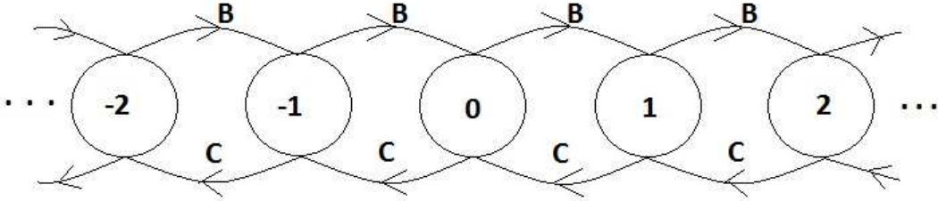
Figure 1. A homogeneous open quantum walk on a line.
