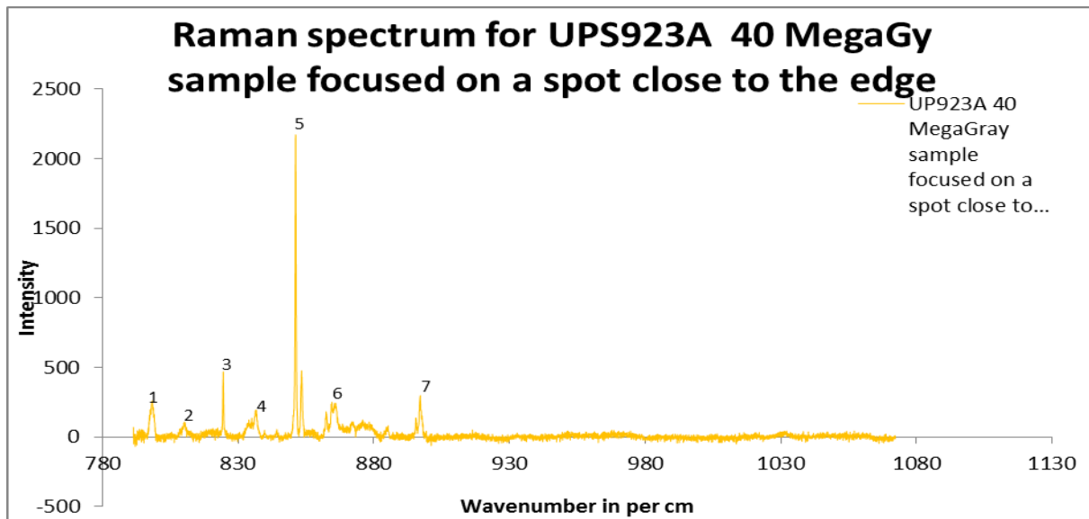
Figure 2. Raman spectrum for UPS923A 40 MegaGy sample.
