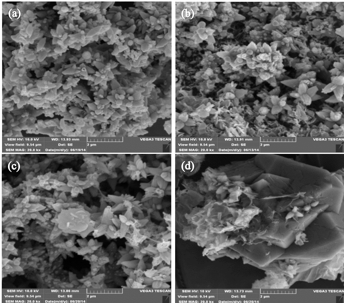
Figure 2. SEM images of ZnO nanoparticles prepared at different concentrations of ZnAc using the CBD method, (a) 0.1 M, (b) 0.14 M, (c) 0.18 M and (d) 0.2 M.
