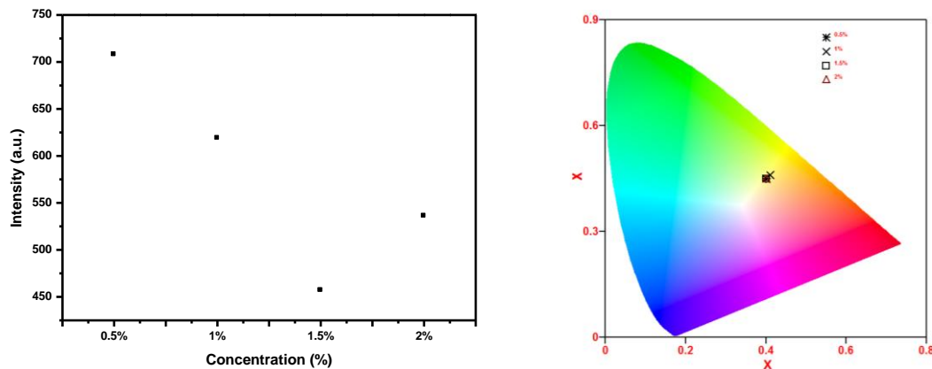
Figure 6. (a) 574 nm PL peak intensity vs concentration graph of the YVO 4 :Dy 3+ phosphor, (b) CIE of YVO 4 :Dy.
