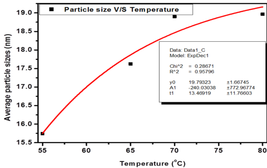
Figure 2. The dependence of average grain sizes of the PbS on the the synthesis temperature of the CBD.
