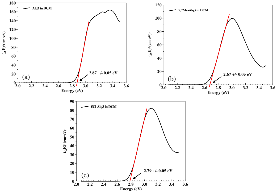
Figure 3: Plot of (\alpha E)^2 versus photon energy ( E ) for (a) \text{Alq}_3 (b) 5,7\text{Me-Alq}_3 and (c) 5\text{Cl-Alq}_3 in DCM.
