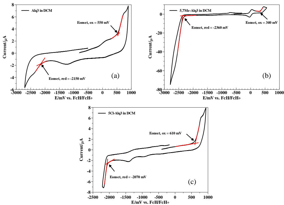
Figure 1: Cyclic voltammograms of (a) Alq 3 (b) 5,7Me-Alq 3 and (c) 5Cl-Alq 3 in DCM.
