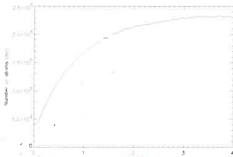
Figure 7. Integrated image intensity of the cloud as a function of time showing growth of the cloud of cold atoms from the time the system is started.
