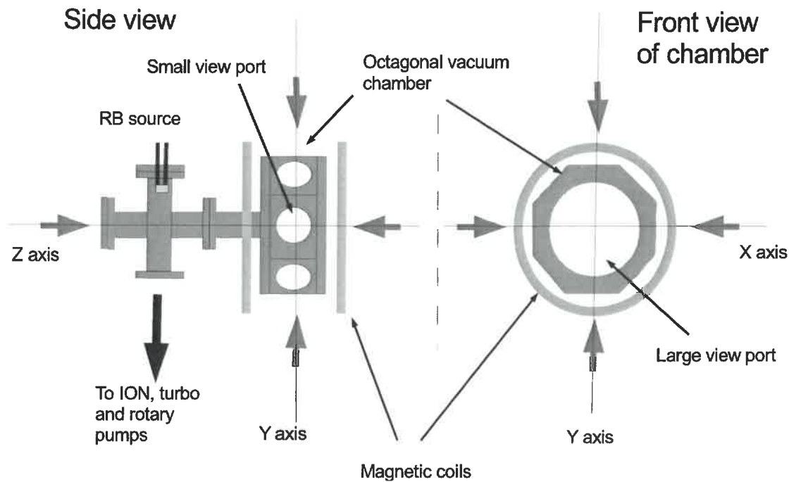
Figure 3. Schematic of the vacuum system. The system consists of an octagonal chamber having a number of view ports on the side and a large view port in front. Also shown in this figure are the counter propagating laser beams (red arrows) entering the chamber along the three axes. Positioned on either side of the chamber is the anti-Helmholtz magnetic coils.
