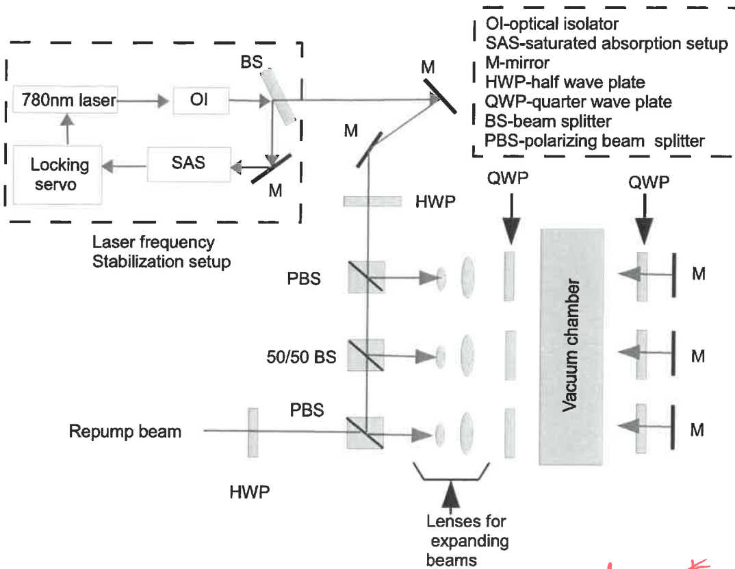
Figure 4. Optical setup.
