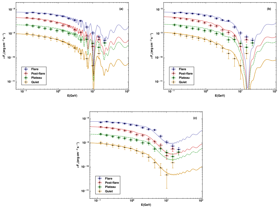
Figure 1. The numerical simulation of the spectral energy fitting observations of blazar 3C454.3 for four different epochs produced using ALP-photon mixing model with electron profile density: (a) n_e \propto R^{-1} , (b) n_e \propto R^{-2} and (c) n_e \propto R^{-3} .
