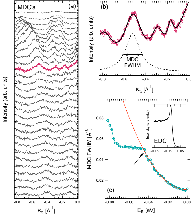
Figure 2. (a) Series of MDC spectra extracted from figure 1b by integrating over an energy range of 10 meV in 2 meV steps. The MDC spectrum in purple symbols is reported separately in (b) together with the overall fitting (solid black line) performed with Lorentzian line shapes. The Lorentzian peak for the band of interest is also reported separately (dashed black line). (c) MDC FWHM for the band of interest in figure 1b plotted versus the binding energy of the peak. The dashed red curve represents a quadratic fit to the low-energy data. The arrow marks the position of the kink. The inset shows a typical energy distribution curve (EDC) for the same peak illustrating the high resolution of these measurements.
