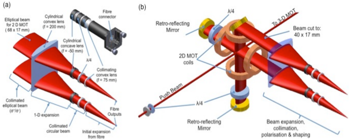
Figure 5: (a) the expansion of the 2-D MOT beam. (b) Illustration showing the magnetic coils and the 2-D + MOT beam configuration.
