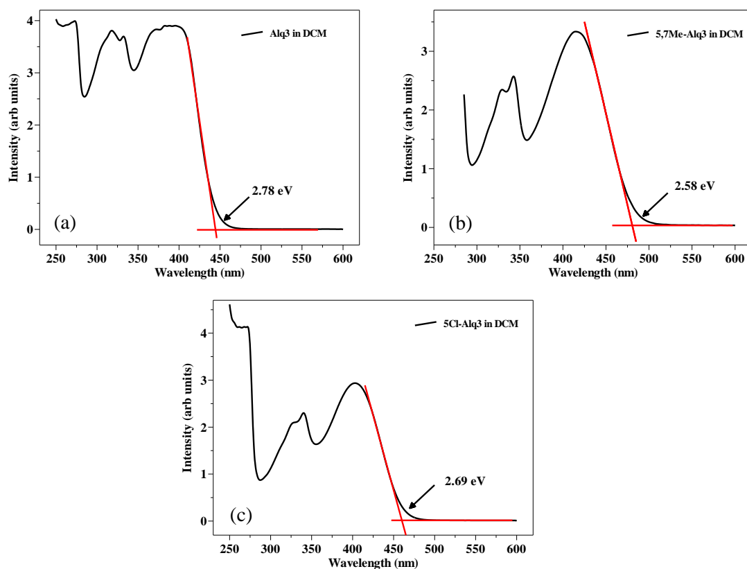
Figure 2: The absorption spectra of (a) Alq 3 (b) 5,7Me-Alq 3 and (c) 5Cl-Alq 3 in DCM. The energy gap is determined from the absorption edges.
