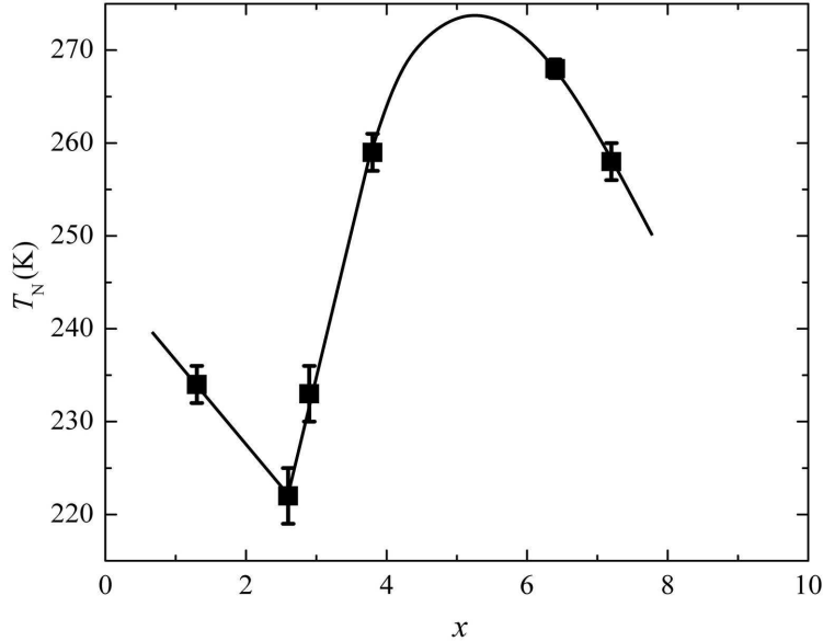
Figure 3. The Néel temperature ( T_N ) as a function of x for the epitaxial \text{Cr}_{100-x}\text{Co}_x thin films prepared on MgO(100).
