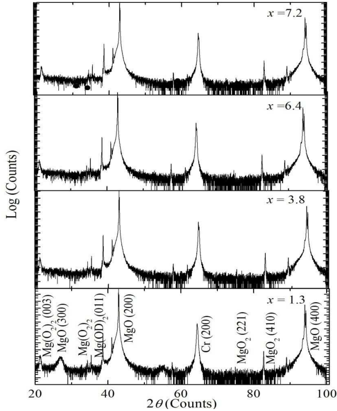
Figure 1. \theta - 2\theta XRD scan (Bragg-Brentano geometry) in which the scattering vector is maintained normal to the plane of the film, for \text{Cr}_{100-x}\text{Co}_x thin films prepared on \text{MgO}(100) substrate.
