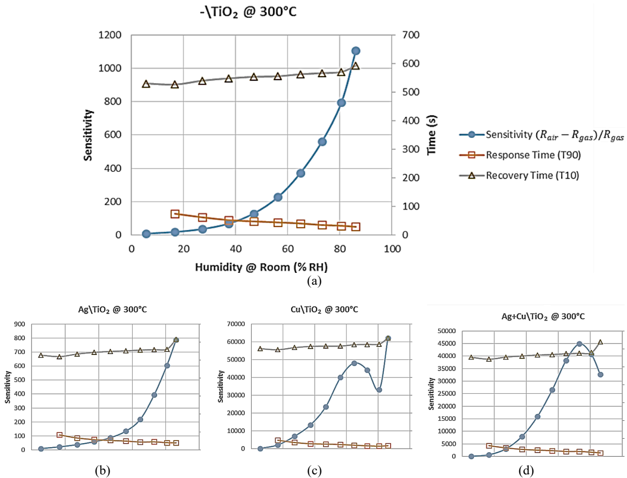
Figure 3. Sensor characteristics of the prepared gas sensors based on (a) the undoped \text{-TiO}_2 , (b) \text{Ag}\text{\TiO}_2 , (c) \text{Cu}\text{\TiO}_2 and (d) \text{Ag+Cu}\text{\TiO}_2 . The anatase nanopowders (annealed at 300^\circ\text{C} ) were exposed to various humidity levels (5.4% RH – 86.1% RH) and measured at room temperature.
