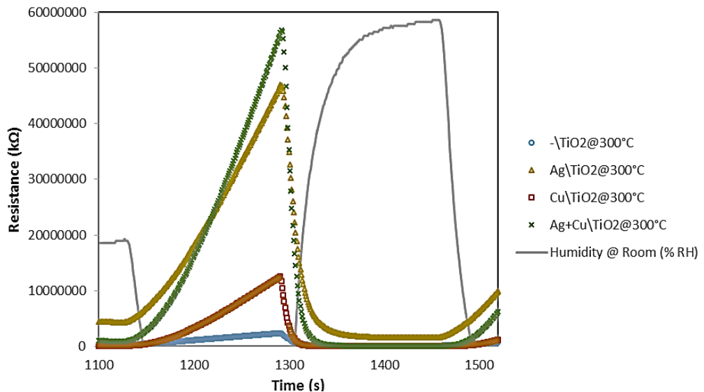
Figure 2. Response-recovery profiles for anatase samples of \text{TiO}_2 , \text{AgTiO}_2 , \text{CuTiO}_2 and \text{Ag+CuTiO}_2 , annealed at 300^\circ\text{C} and exposed to room-temperature humidity of 16.7% RH.
