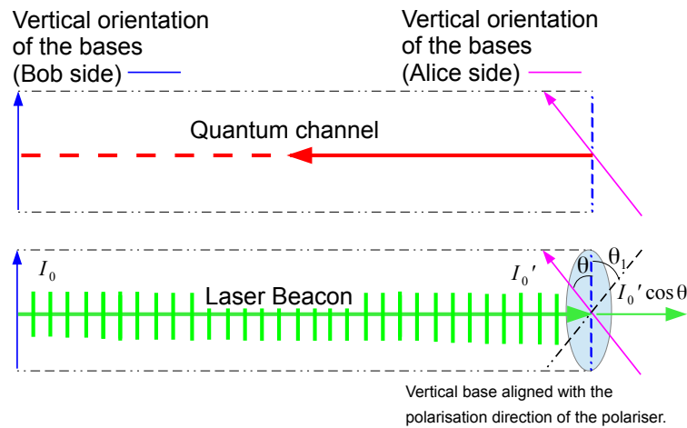
Figure 1. The blue dashed line and the green lines, correspond to the vertical direction of the laser beacon and the violet arrow correspond to the direction of the vertical polarization base of Alice. The vertical polarization direction of Alice is orientated in the same direction of the polariser of the alignment system. The black dashed line represents the ambiguity between the real angle of misalignment \theta and the specular angle \theta_1 . When the laser crosses the polarizer the intensity in output follows the equation (1) from which is possible calculate the angle of misalignment without information of the verse of rotation ( \theta or \theta_1 ).
