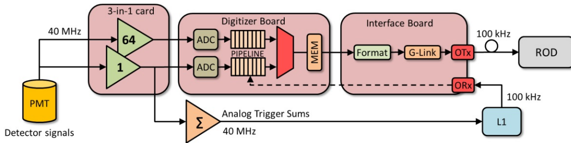
Figure 2: Present Tile Calorimeter readout architecture.
