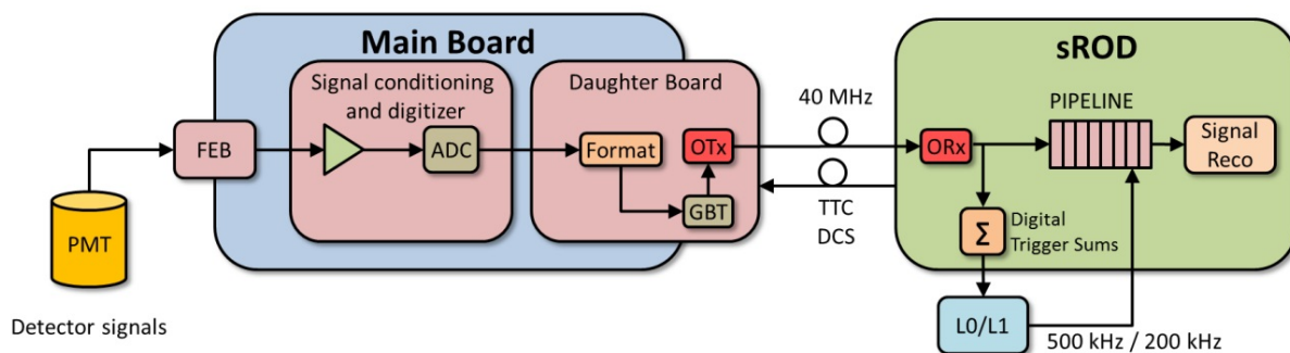
Figure 3: Upgraded Tile Calorimeter readout architecture.
