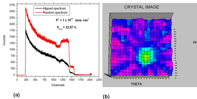
Figure 3. (a) RBS random and aligned spectra, and (b) Channeling crystal image of the InGaN thin film sample at P^+ ion fluence of 1 \times 10^{14} \text{ ions/cm}^2
