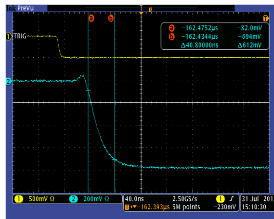
Figure 2. The input pulser (yellow) and the output preamplifier response (blue) signals as observed on an oscilloscope for the core of crystal A.
