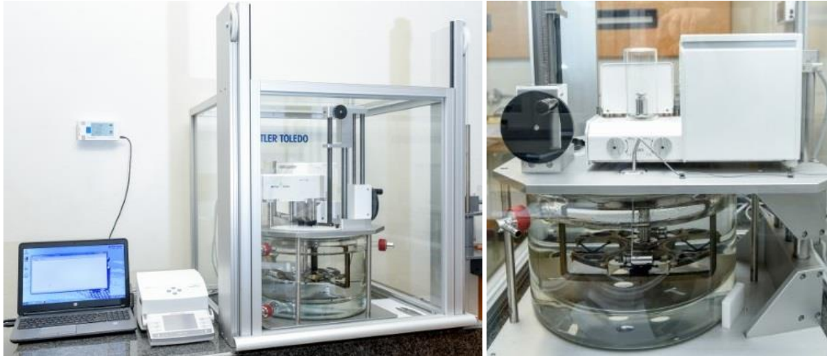
Figure 3: The front view (left) of the VC1005 and the side view (right) of the fluid bath on the right.
