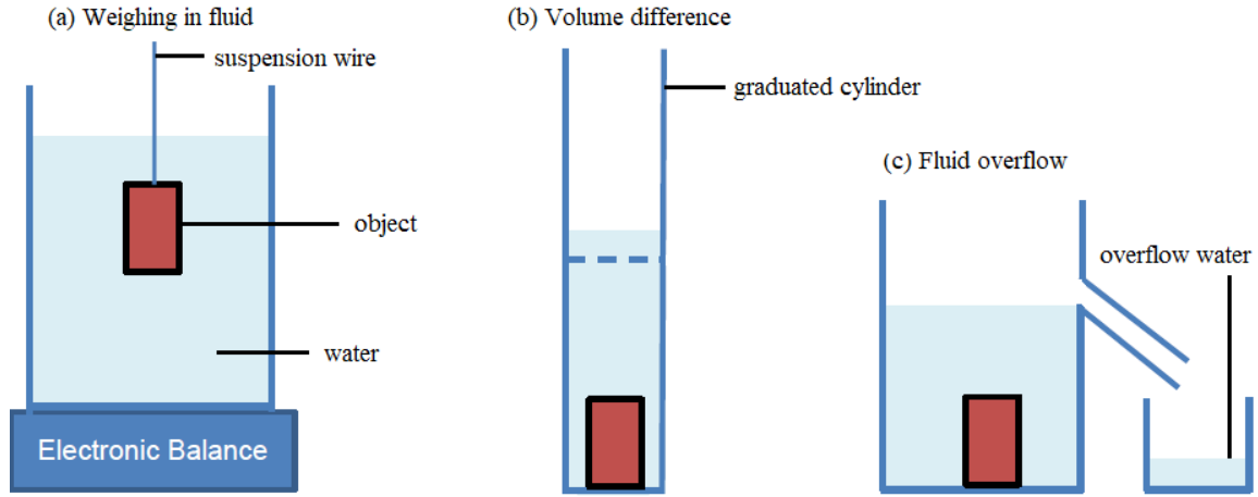
Figure 1: Schematic representation of (a) suspension, (b) liquid level and (c) overflow techniques for volume determination of solids [2].
