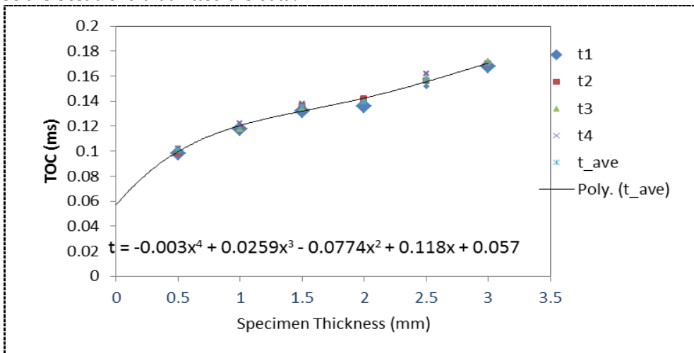
Figure 5. Experimental results: Thickness versus Time of Crossing (TOC)
