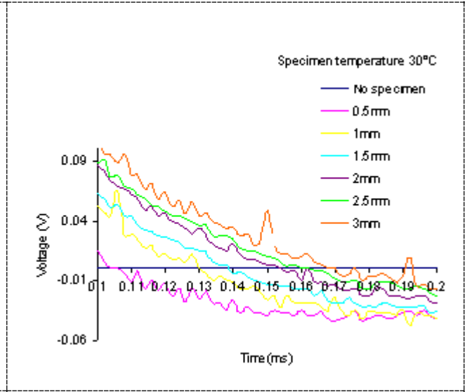
Figure 5. Zero Crossing is Time of crossing (TOC)
