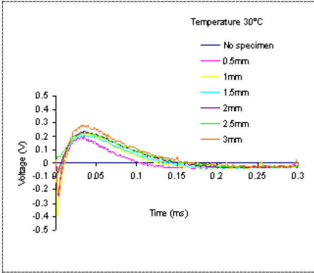
Figure 4. Difference signals
