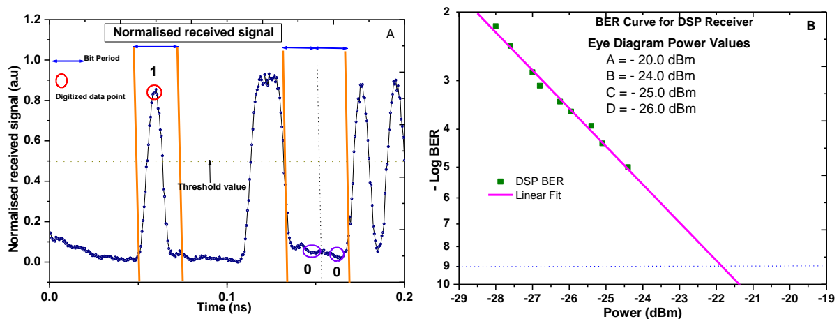
Figure 3: A. DSP normalised and digitized signal as captured from the digital storage oscilloscope B. DSP back to back BER curves for different received optical powers.
