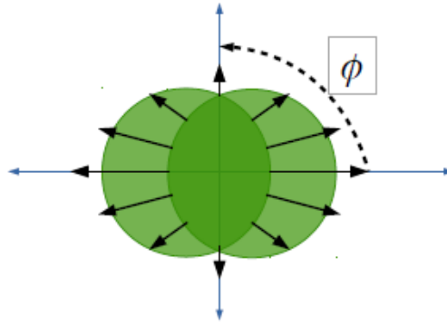
Figure 1. The overlap region of two nuclei as seen in the plane transverse to the beam and the azimuthal angle \phi as measured in the event plane. Black arrows indicate the emission of high-momentum particles in plane ( \phi \sim 0, \pi ) and lower-momentum particles out-of-plane ( \phi \sim \frac{\pi}{2}, \frac{3\pi}{2} ). (Drawn by author)
